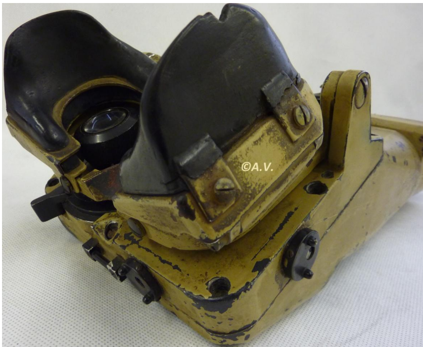
Pict 33; 12x60 bpd model; openings adjustment for centralizing reticle ©Anna Vacani
